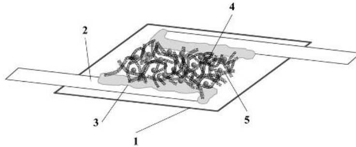
Figure 1. Scheme of a device used for hydrogen detection. (1) Non-conductive support; (2) Adhesive metal tape; (3) Conducting paint; (4) CNT deposit; (5) Metal nanoparticles
