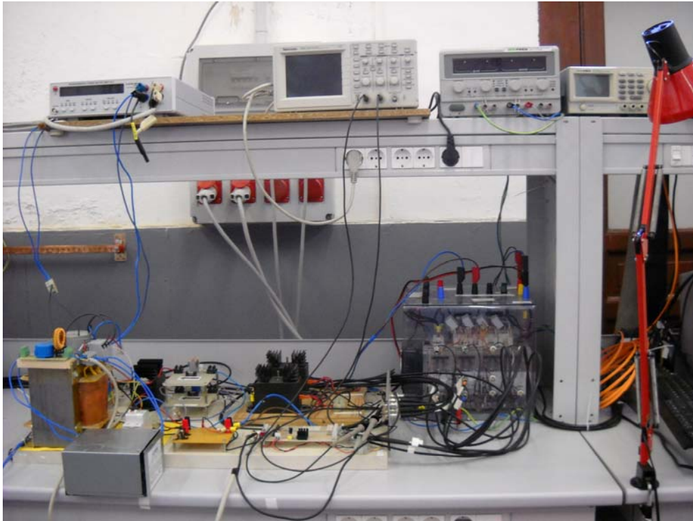
Micro-WECS: circuit
