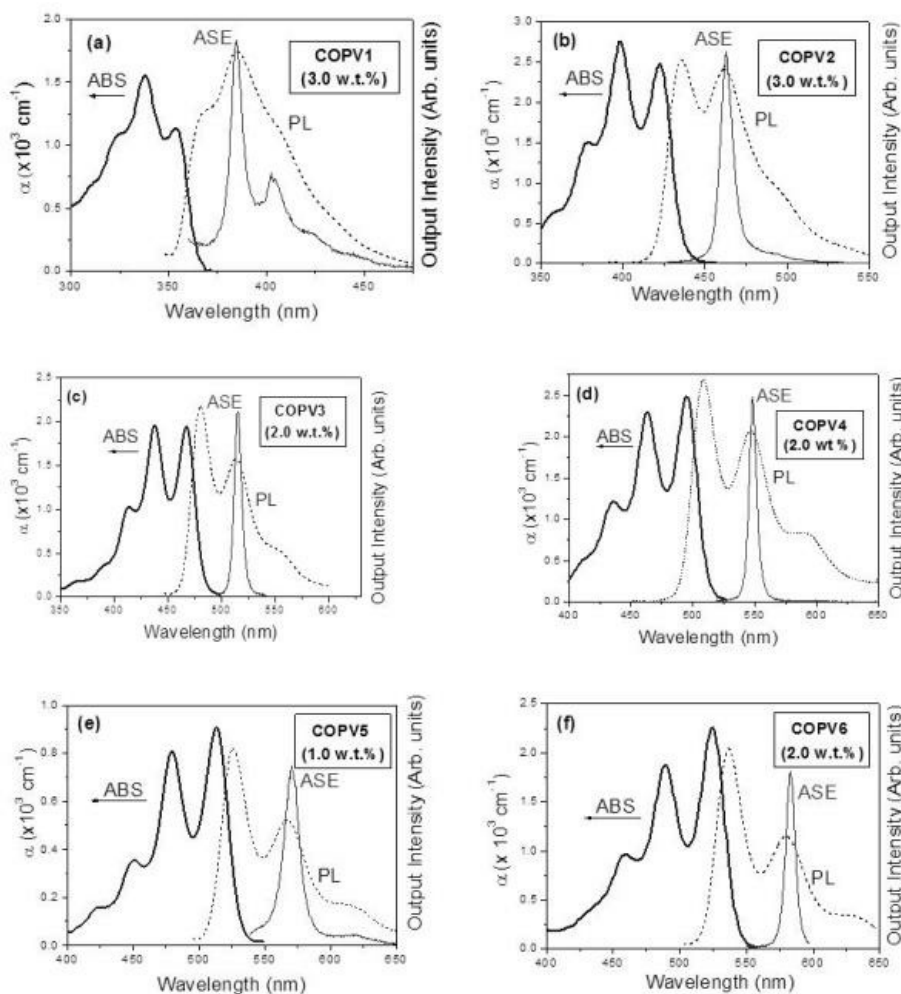
Figure 3. Following figures, from a) to f), show the absorbance (ABS, thick solid line, left axis), photoluminescence and ASE (PL, dashed line and thin solid line, respectively; right axis) spectra for PS films containing a COPVn derivative, for n = 1 to 6, respectively (doping rate indicated in the legend) deposited over bare fused silica substrates (without gratings);
