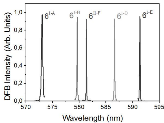
Figura 5. This figure shows the emission spectra of various DFB lasers based on PS films containing COPV6, aiming to illustrate the capability of tuning the emission wavelength for a given COPV derivative, by changing the device active film thickness or the grating period.
