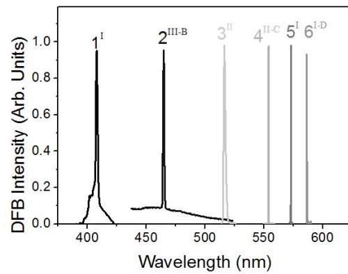
Figura 5. This figure shows the emission spectra of various DFB lasers based on PS films containing COPV6, aiming to illustrate the capability of tuning the emission wavelength for a given COPV derivative, by changing the device active film thickness or the grating period.
